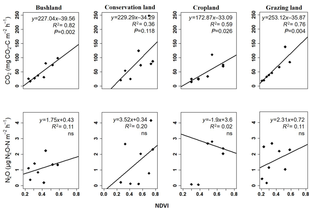
Figure 7. Linear regression analyses of the measured seasonal means for soil \text{CO}_2 and soil \text{N}_2\text{O} emissions during the campaign from November 2017 to November 2018 plotted against NDVI data acquired during each campaign; ns = not significant.
