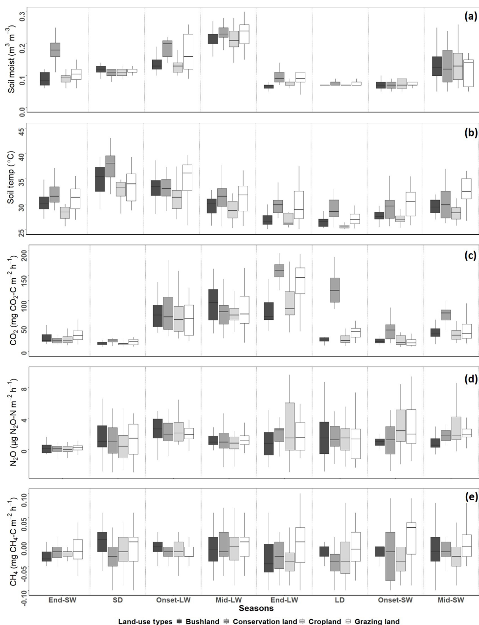
Figure 4. Box plots showing differences in seasonal means for (a) soil moisture and (b) soil temperature and for soil emissions of (c) \text{CO}_2 , (d) \text{N}_2\text{O} , and (e) \text{CH}_4 for each site from November 2017 to October 2018. Season abbreviations on the x axis are SW for the short wet season and LW for the long wet season, with onset, middle (mid) and end of the corresponding wet season also shown, along with SD for the short dry season and LD for the long dry season.
