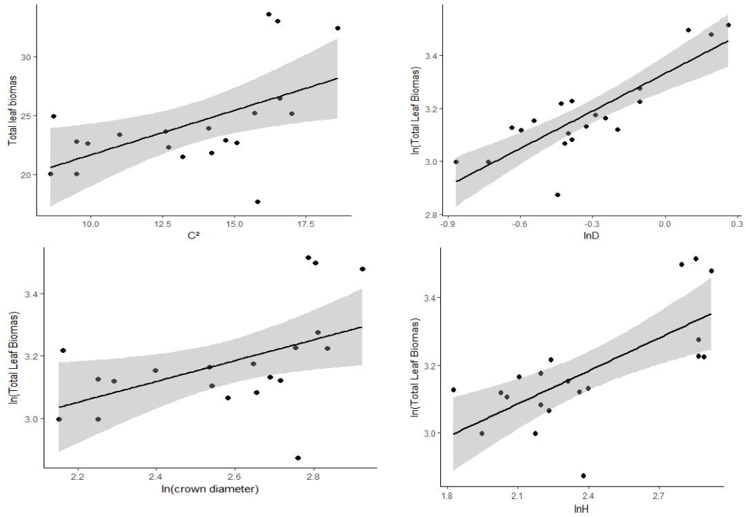
Fig. 3a. Scatter diagrams of F. albida leaf biomass fitted models 1 to 6
