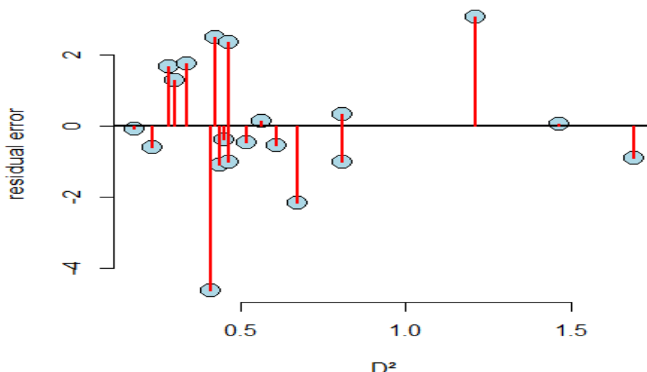
Fig. 4. Residual distribution of model 1
