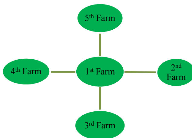
Fig. 2. Sampling design for F. albida
