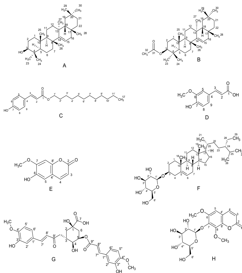
Figure 1. Structures of compounds isolated from A. afra roots (A–H).
