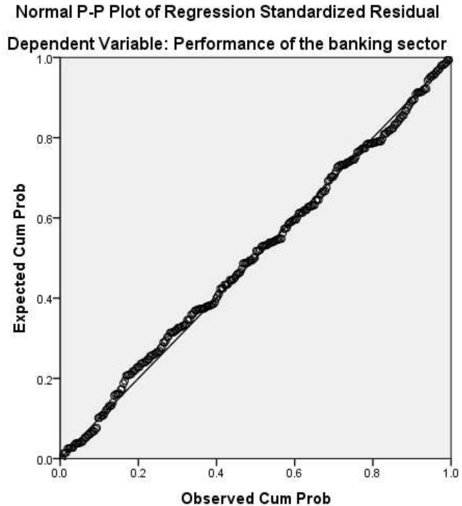
Figure 3.1: Normality test
