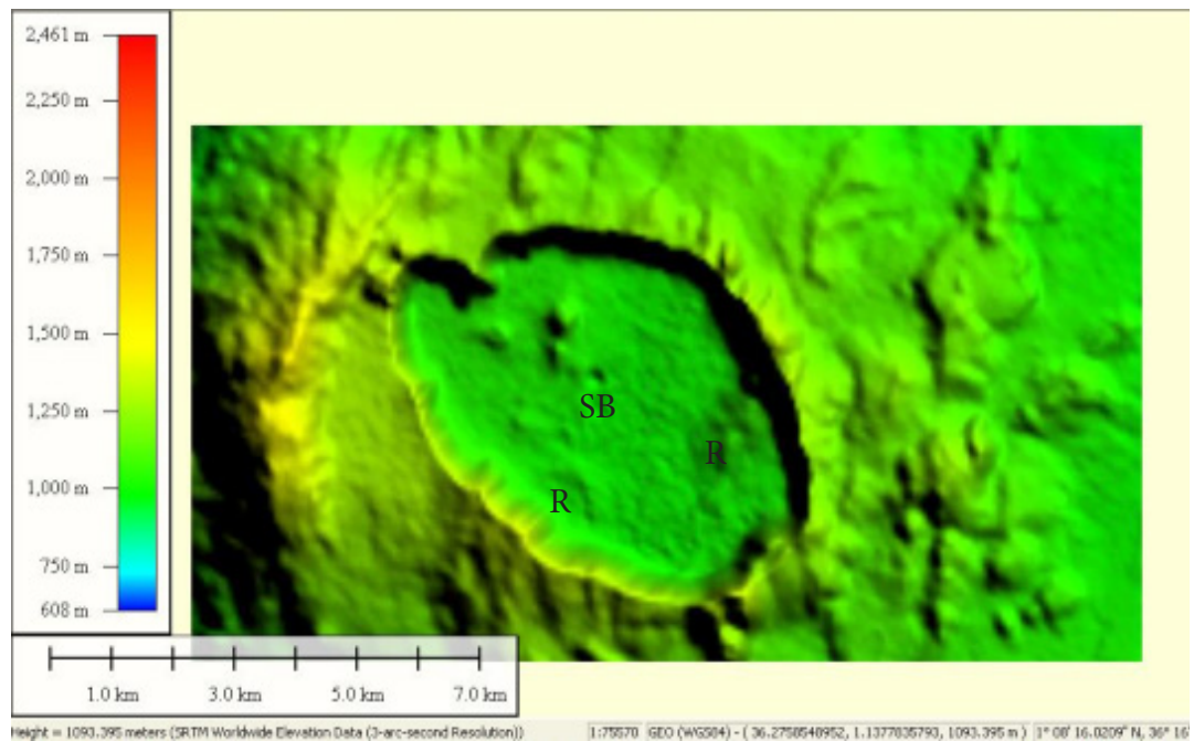
Plate 6 A DEM (with elevations) showing Silali basin's (SB) hummocky terrain and morphology. The DEM also shows the outline of Silali's probable peak ring (R) (Author, 2015).
