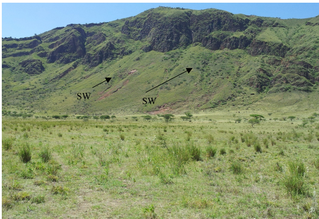
Plate 14: A picture showing more of Silali basin's slumped inner walls (SW) (Author 2015).
