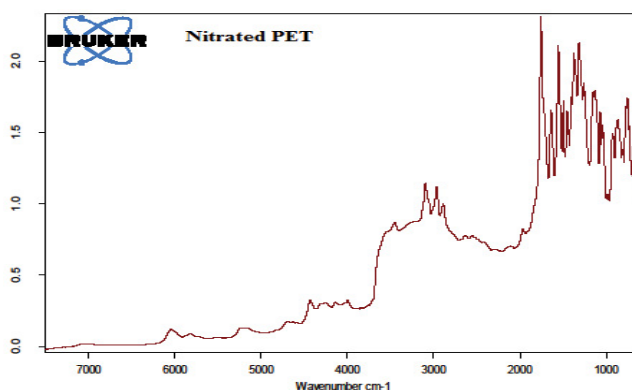
Figure 2: FTIR spectrum of the nitrated PET
