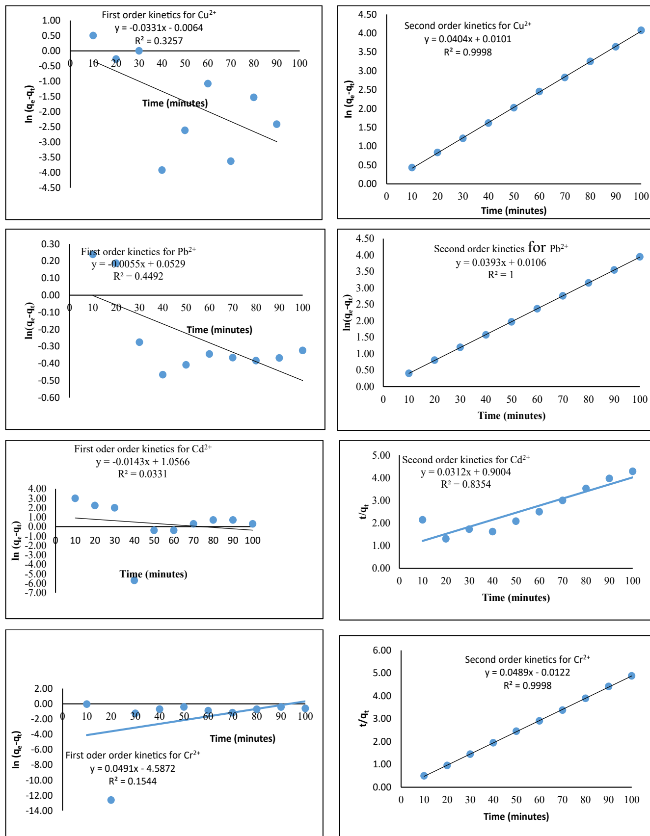
Figure 9: Kinetic data on the sorption of metal ions
