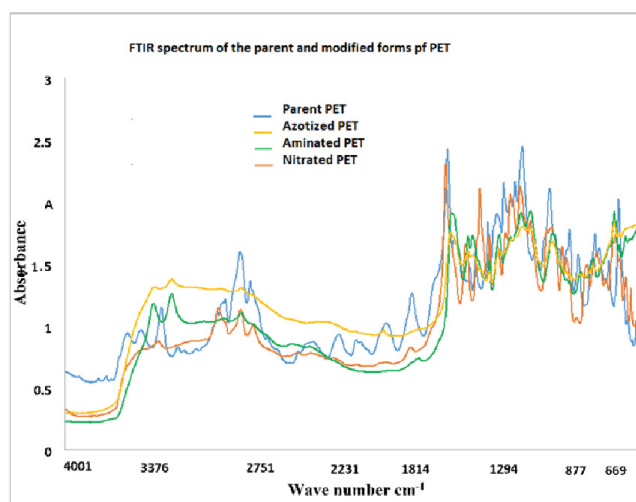
Figure 5: FTIR spectrum of the parent PET and its modified forms
