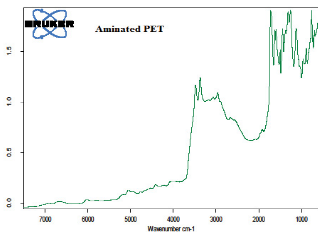
Figure 3: FTIR spectrum of the aminated PET
