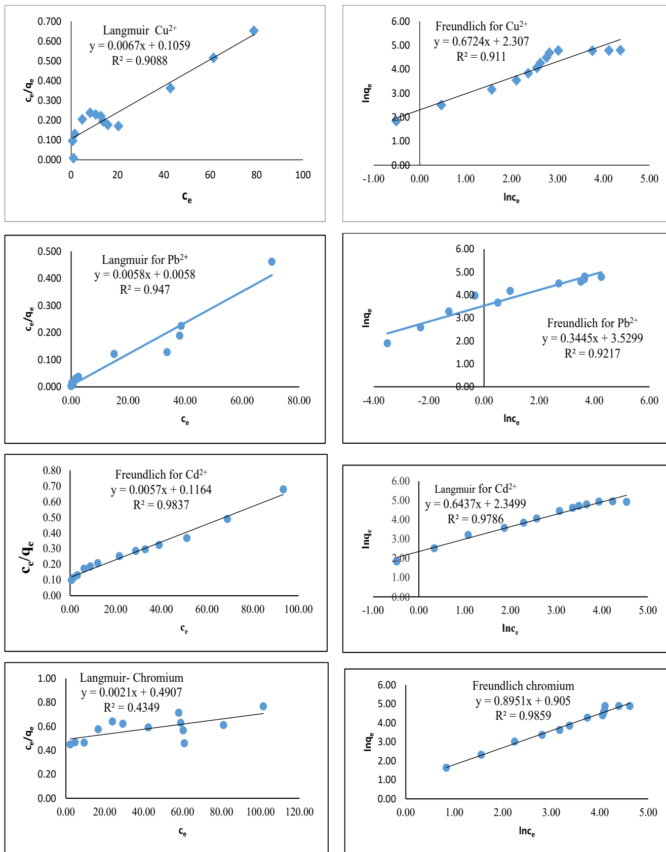
Figure 11: Adsorption isotherms for some selected metal by azotized PET
