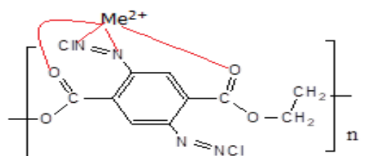
Scheme 1: Metallized azo pigment
