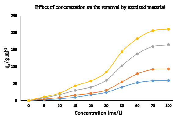
Figure 8: Effect of initial metal ion concentration on the sorption of metal ions
