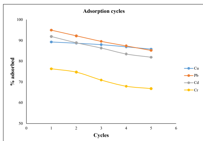
Figure 12: Adsorption cycles of the azotized PET for the metal ions.
