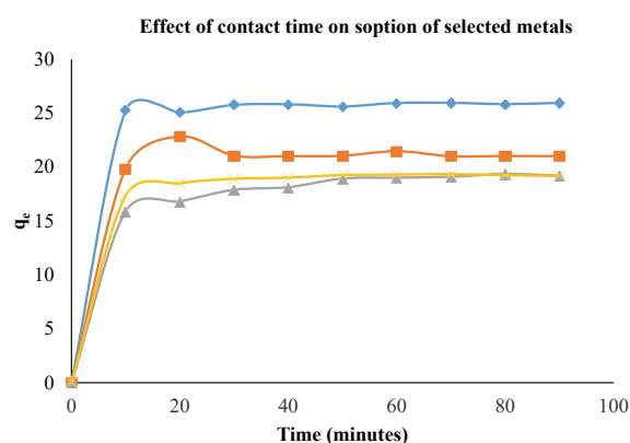
Figure 7: Effect of contact time on the adsorption of metal ions
