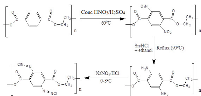
Scheme 2: Azotization of the polyethylene terephthalate material
