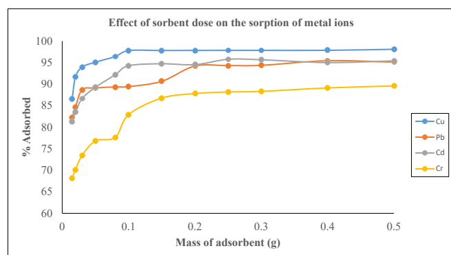
Figure 10: Effect of sorbent dose on the sorption of metal ions
