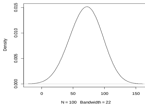
Fig. 7 Arbitrary bandwidth of 22
