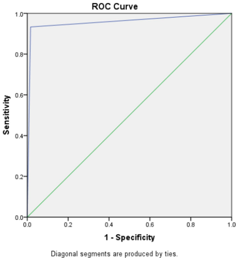
Fig. 2 ROC curve analysis for HbA2 hemoglobin
