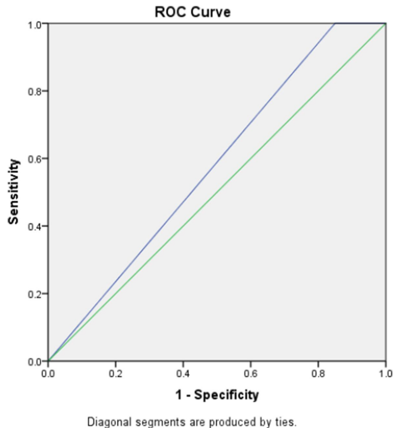
Fig. 1 ROC curve analysis for current HbA normal range of 95–98%
