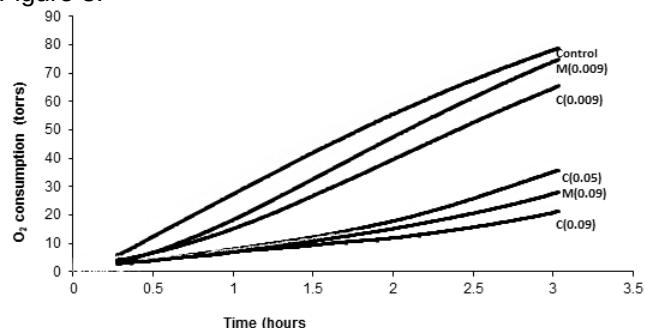
Figure 3: Antioxidant properties of (-)-mesquitol (M) and (+)-catechin (C) at different concentrations(g/l) estimated using methyl linoleate oxidation inhibition
