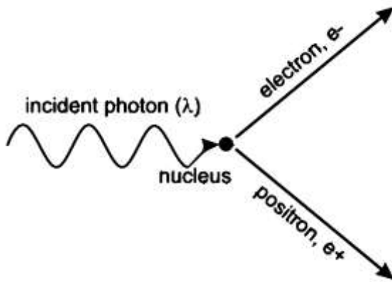
Figure 2.4: A schematic diagram showing the formation of an electron-positron pair (Ragheb, 2011).
