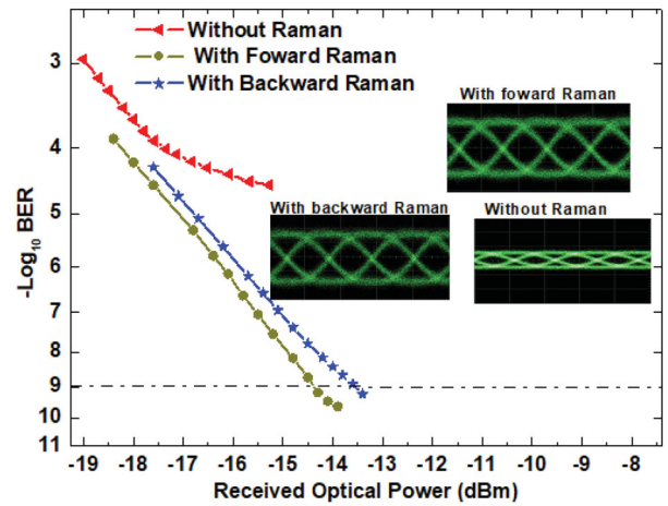
Figure 7. Bit error rate (BER) curve for 8.5 Gbps VCSEL performance at back-to-back (B2B) and 50.7 km Raman-assisted fibre transmission.
