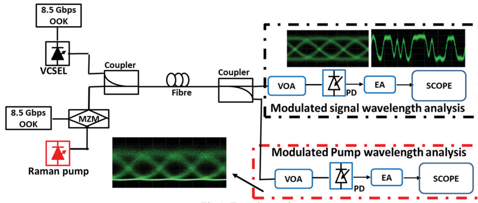
Figure 1. Experimental setup.
