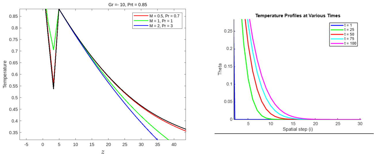
Figure 4.6 Temperature profiles
