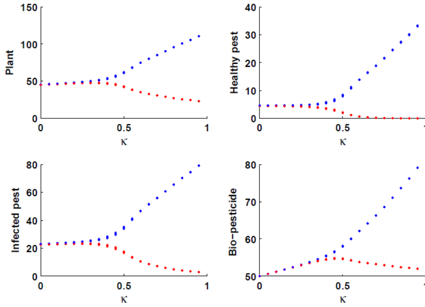
FIGURE 5. System dynamics for varying \kappa and parameter are as given in Table 1.
