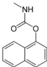
Figure 2.10: Structural formula of carbaryl
