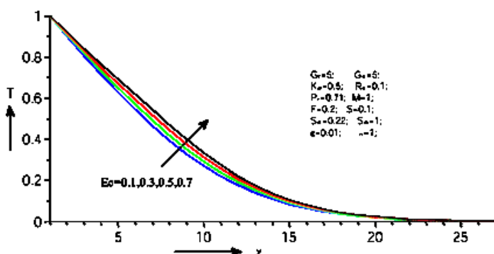
Figure 4.7 Effect of Eckert number on temperature
