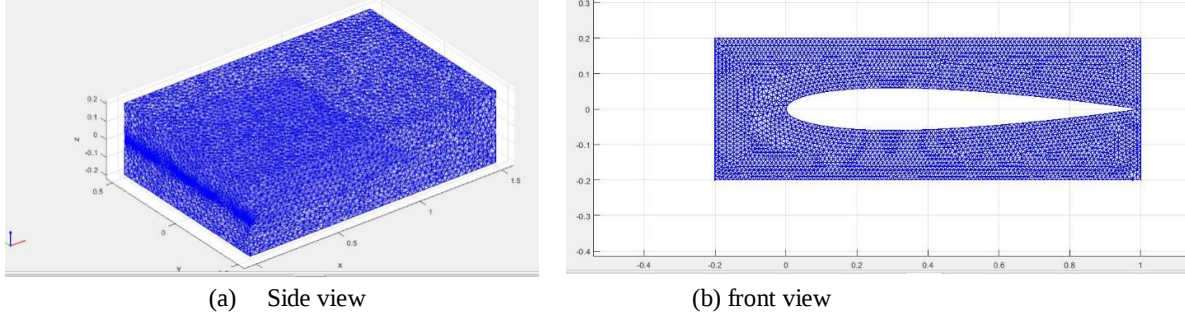
Figure 4.2 Grid generations of Porous Wings
