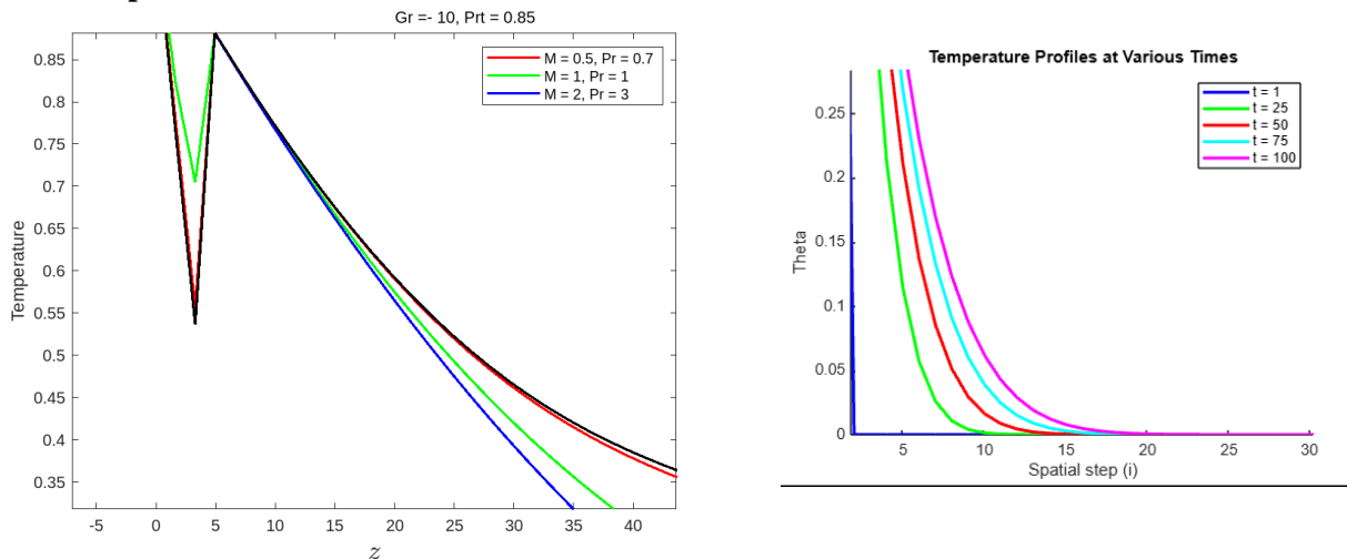
Figure 4.6 Temperature profiles
