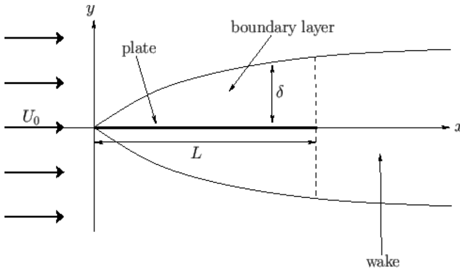
Figure 1.2 Flow over a flat plate
