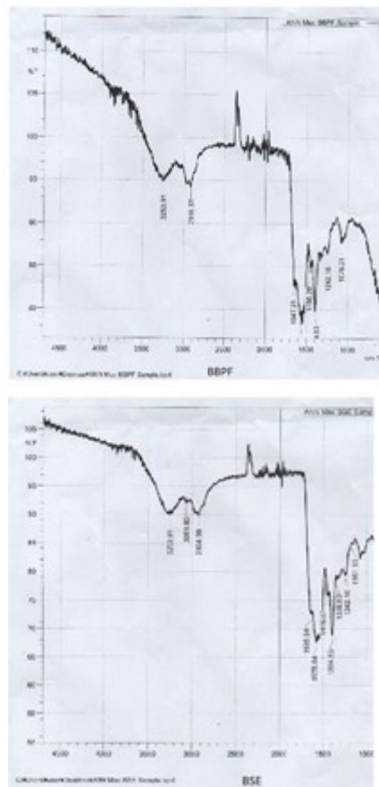
Figure 1: Fourier Transform Infrared spectra for the Red snapper, Blue barred parrot fish and Black spot emperor respectively.
