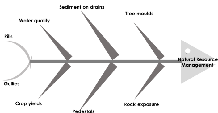
Fig. 1. An illustration on the association between soil erosion monitoring indicators and natural resource management
