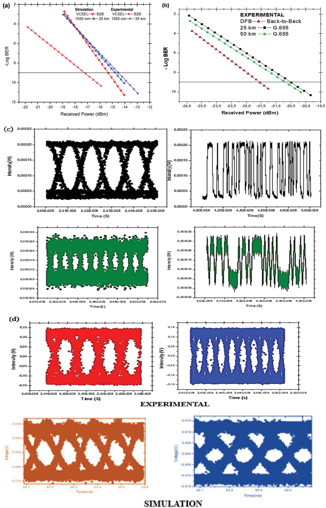
Figure 3. (a): Simulation and experimental plots of -\text{Log BER} curves of B2B and 25 km transmission using 10 Gbps 1550 nm VCSEL. (b): Experimental -\text{Log BER} curves for B2B, 25 and 50 km WDM DFB transmission on a G.655 fibre. (c): Eye diagrams and resultant waveforms for 25 km (black) and 50 km (green) transmission using a DFB. (d): Experimental and simulated eye diagrams for B2B (orange) and 25 km transmission (blue) using a VCSEL and G.655 fibre.
