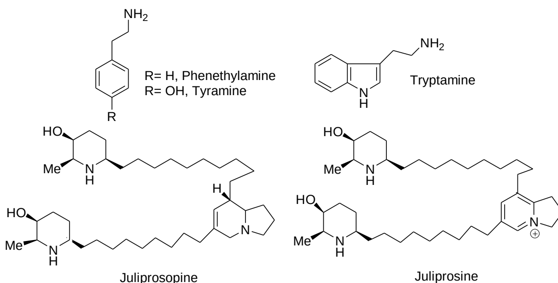
Figure 3. Some components contained in leaf extractives of P. juliflora
