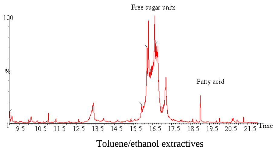
Figure 6. GC-MS chromatograms of the different compounds in pods extractives
