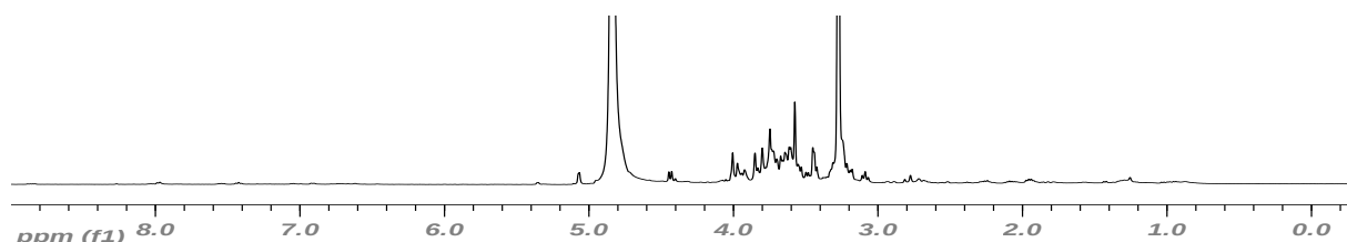
Figure 4. ^1\text{H} NMR analysis for P. Juliflora whole pod extractives
