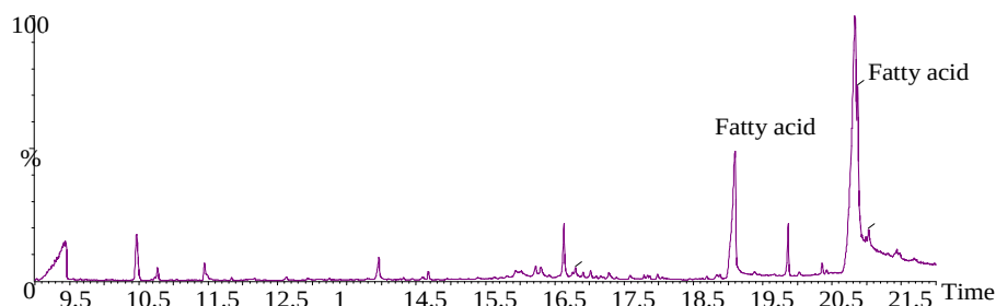
Dichloromethane extractives
