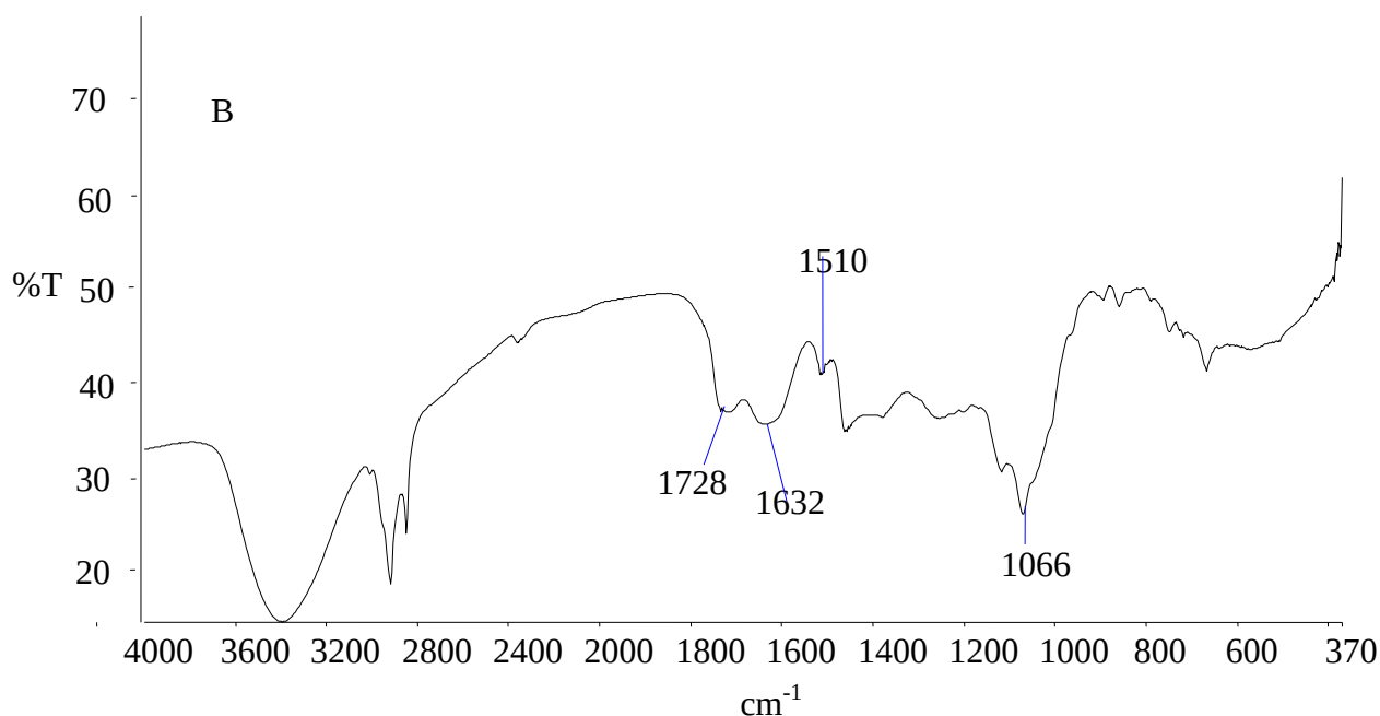
Figure 2. FTIR spectrum of (A) toluene/ethanol and (B) acetone extractives of P. juliflora leaves
