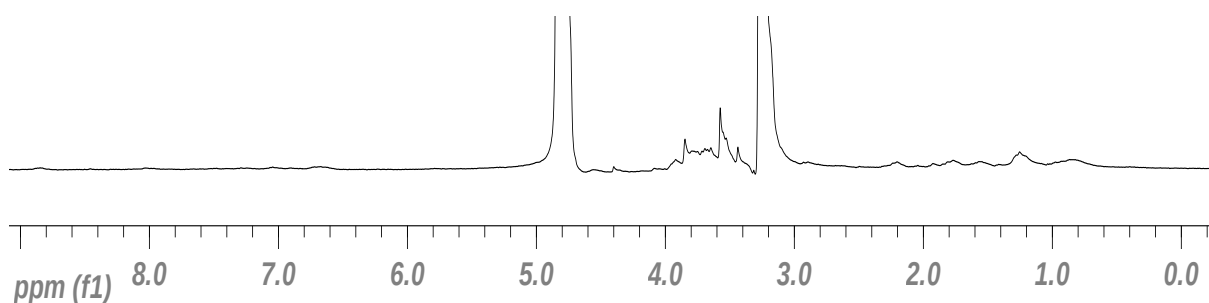
Figure 1. ^1\text{H} NMR analysis for P. Juliflora leaves extractives by different solvents
