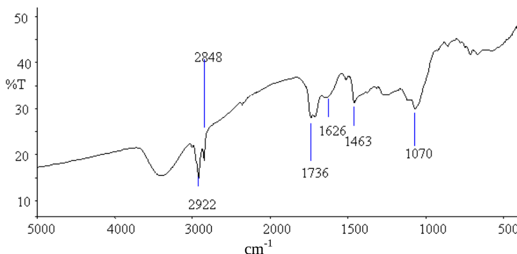
Figure 5. FTIR spectrum for pods dichloromethane extractives
