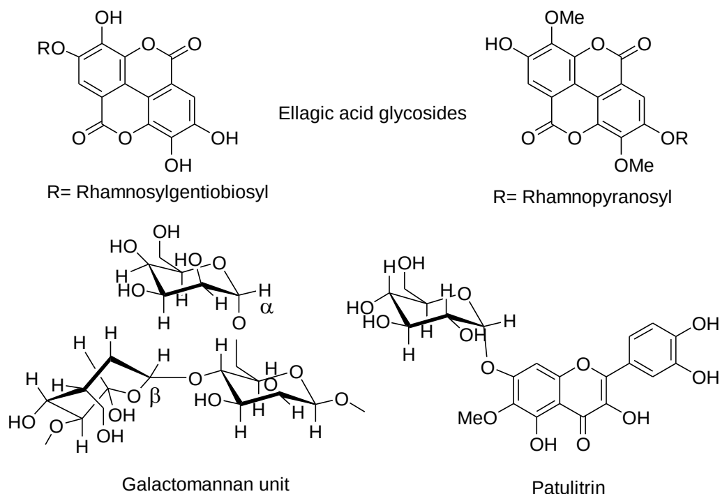
Figure 7. Some components contained in pods extractives of P. juliflora
