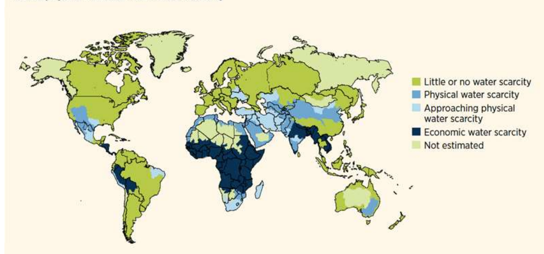
Global physical and economic water scarcity
