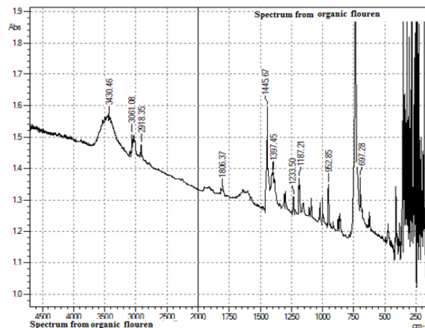
Fig. 8. FTIR absorption spectrum from flourene fluorescent organic material
