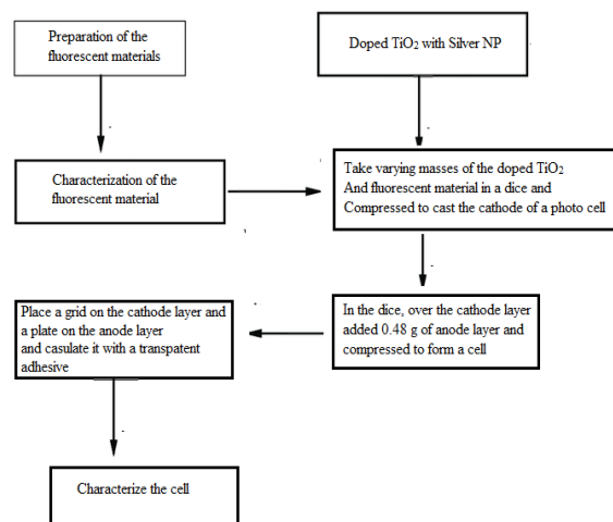
Fig. 1. Flow diagram of the solar cell fabrication process
