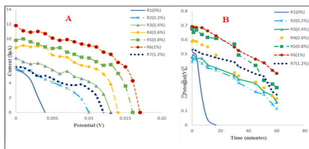
Fig. 7. Characterization of Ag-enhanced titanium dioxide doped with gingerol (A) I-V, (B) P-T
