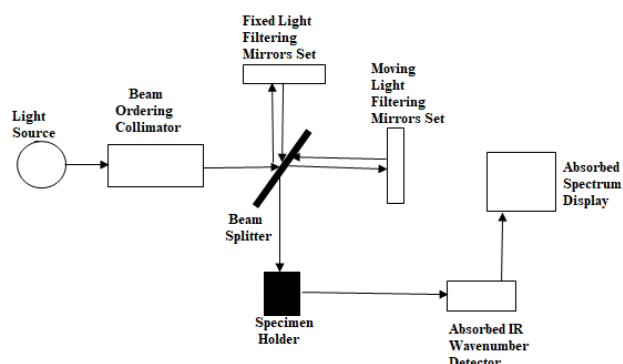
Fig. 2. Schematic presentation of a Fourier-transform infrared spectroscopy
