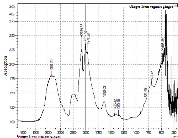
Fig. 6. FTIR absorption spectrum analysis of Gingerol luminescent material
