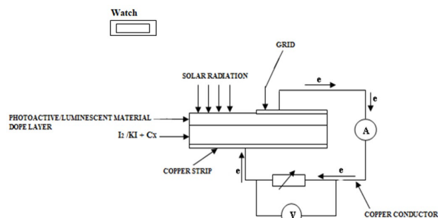
Fig 3. Schematic presentation of the cell characterization circuit
