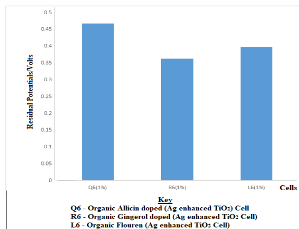
Fig. 10. Residual Potential against \{Q_6(1\%), R_6(1\%) \text{ and } L_6(1\%) \} (Ag enhanced titanium dioxide) FSCs
