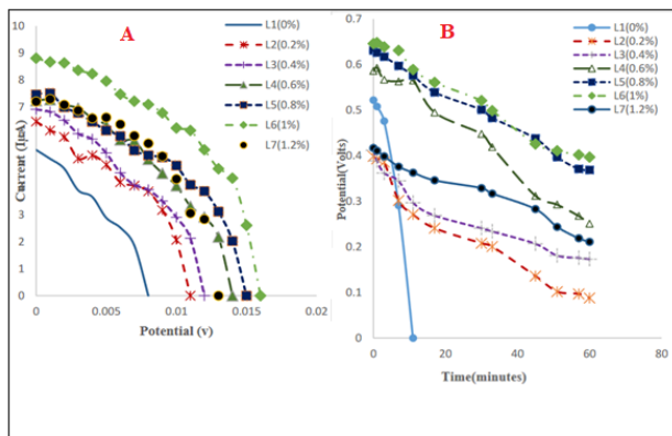
Fig. 9. Characterization of Ag-enhanced titanium dioxide doped with fluorene (A) I-V, (B) P-T
