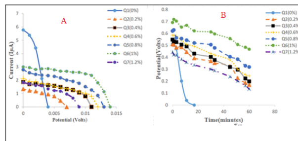
Fig. 5. Characterization of Ag-enhanced TiO 2 doped with allicin (A) I-V, (B) P-t
