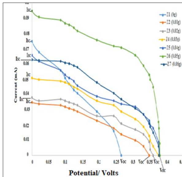
Figure 6 I-V characterization for (Sb/Ca/Mn*Ag) \text{TiO}_2 Fluorescent cells at constant (0.25 g) \text{TiO}_2
