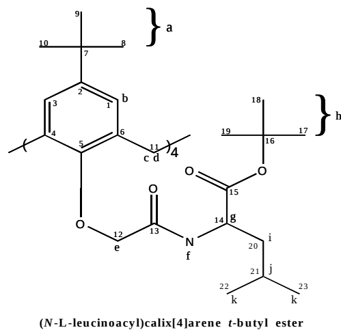
Figure 2. Structures of ( N -L-aminoacyl)calixarenes.
