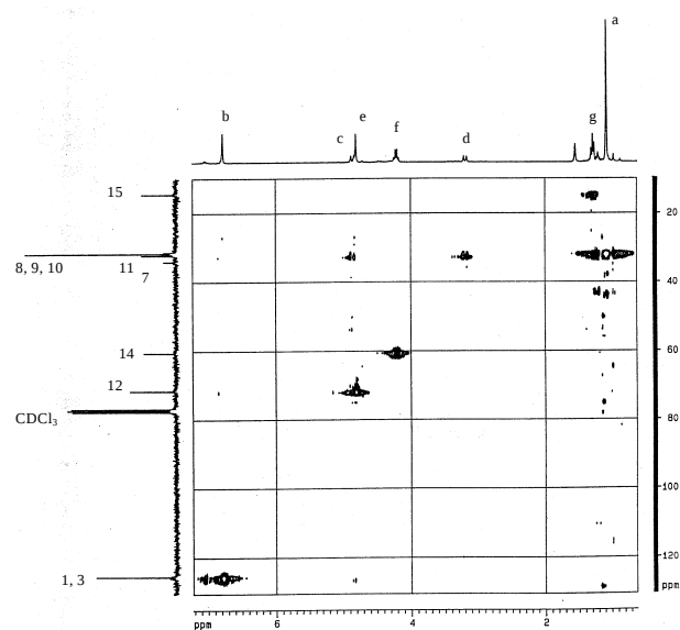
Figure 4. HMQC spectrum of calixaryl ester (Compound 2).
